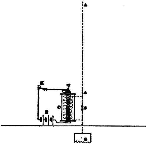
FIG. 32.—Elements of Connections at Sending Station.
